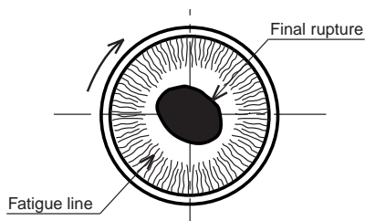
Torsional fatigue
